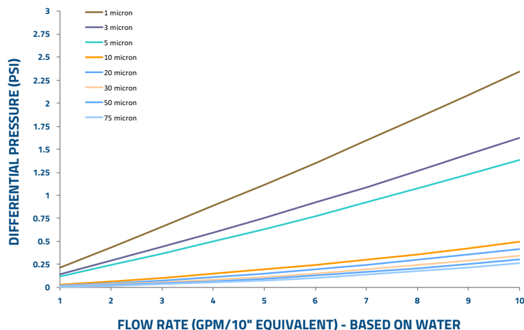
KLARES SILVER SERIES DP vs FLOW RATE
