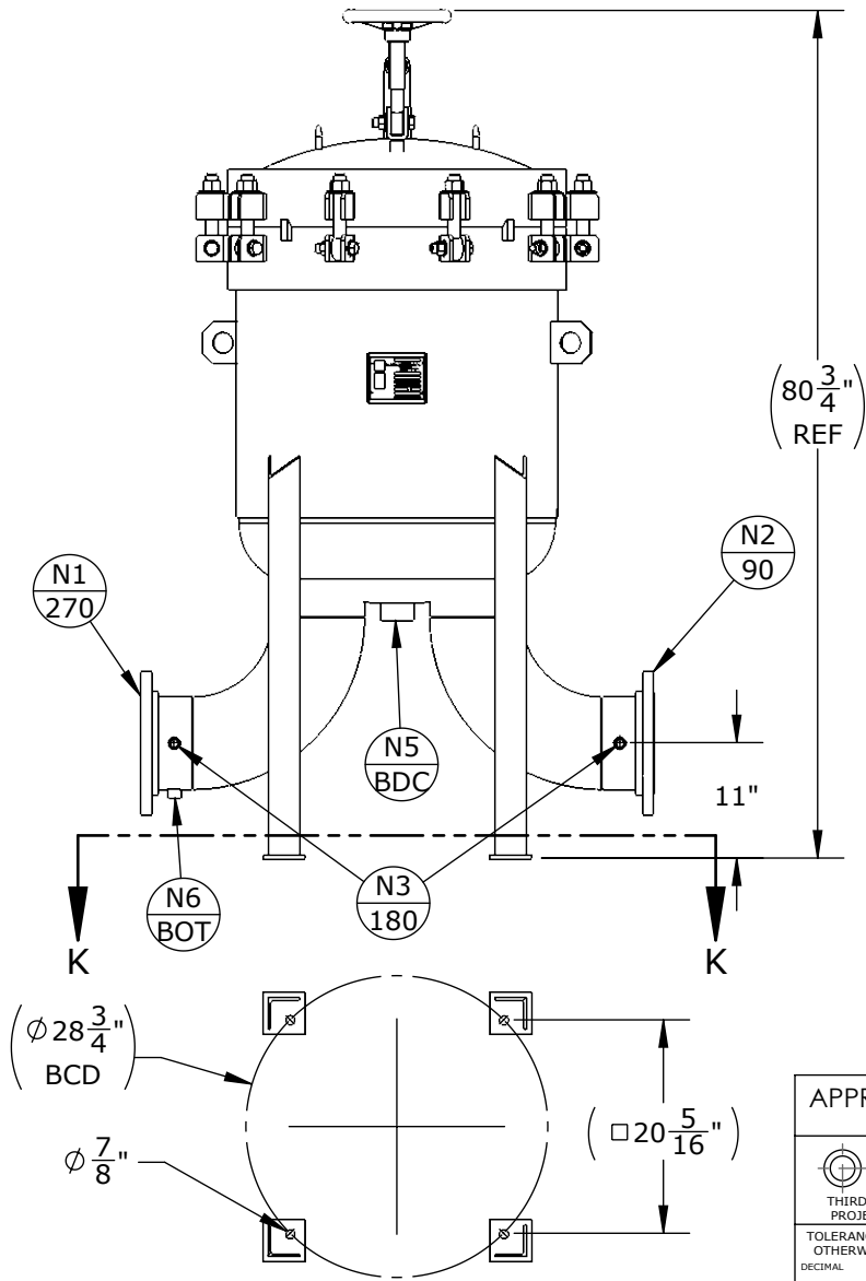
SECTION K-K SCALE 1 : 20
