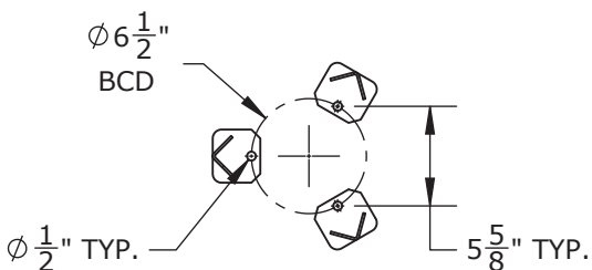
SECTION M-M
