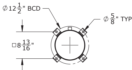
SECTION K-K SCALE 1 : 16
