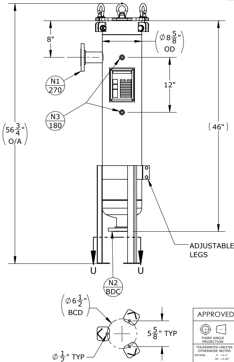
SECTION U-U SCALE 1 : 12
