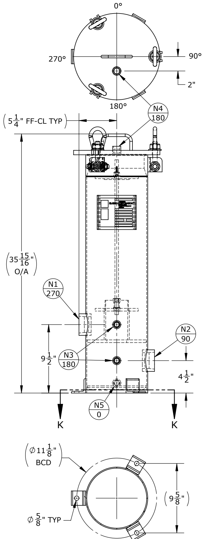
SECTION K-K
