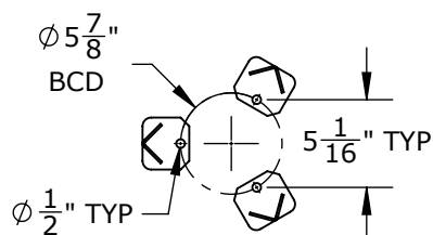
SECTION K-K
