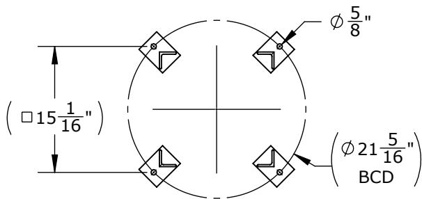
SECTION K-K
