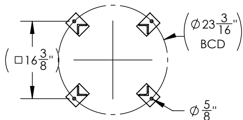
SECTION M-M SCALE 1 : 20
